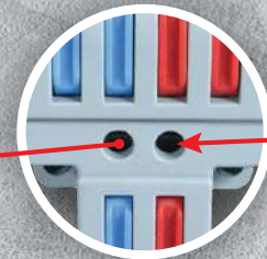
Points for Voltage Testing
